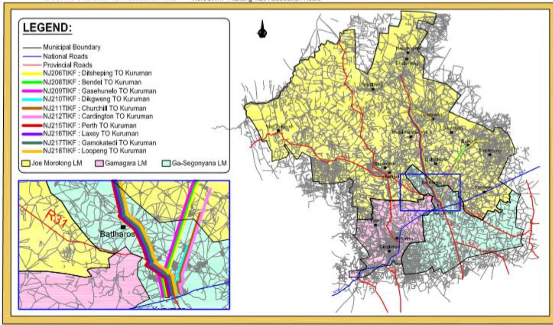
Figure18(i):Taxi routes
